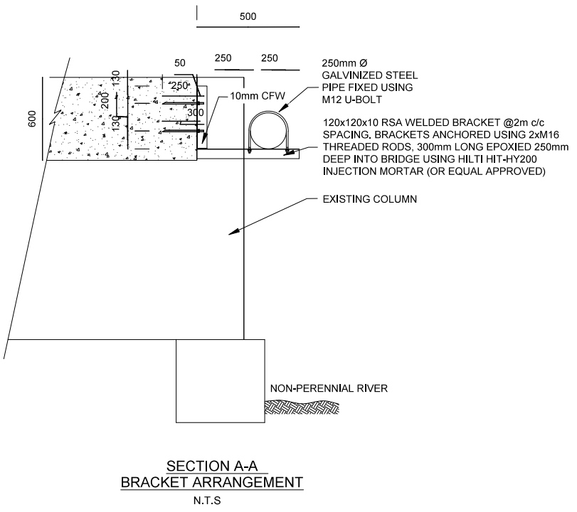
PIPE BRIDGE CROSSING MH 241-MH 242
